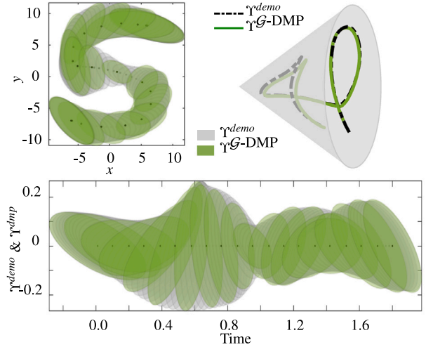
Fig. 8. Top-Left : The Cartesian trajectory (in centimeters) executed by the 5-DoF manipulator (black dots), the demonstrated manipulability profile (gray ellipses), and the manipulability profile learned by \mathcal{G} -DMP (green ellipses), shown at different times during the execution of the task. Top-Right : Representation of SPD manifold (gray cone) containing the demonstrated (dashed black line) and learned (green solid line) manipulability profiles. Bottom : Variation of demonstrated (gray ellipses) and learned (green ellipses) manipulability profiles over time.
