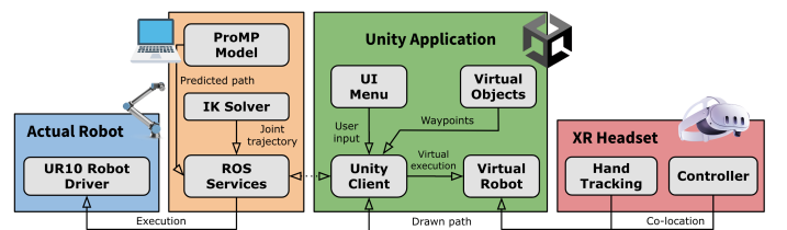
Fig. 5. Technical workflow of RAMPA.
